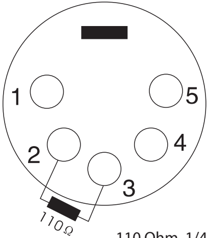
110 Ohm, 1/4 watt resistor soldered on pins 2 & 3
